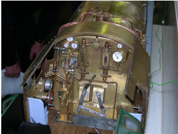
Backhead Details
