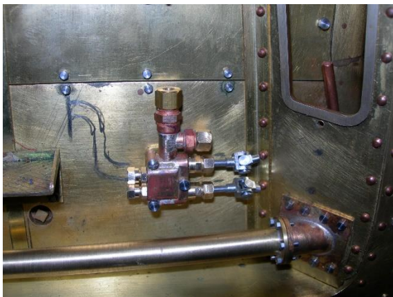
Ejector Valves
