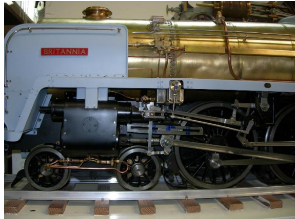
Cylinder and Smoke Deflector
